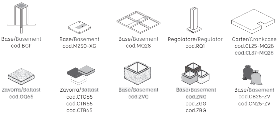
BASI E ZAVORRE / BASES AND BALLASTS
